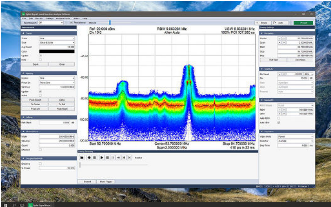
Figure 3—Spectrum analyzer software running on a PC
