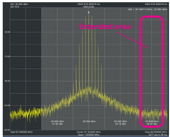
Figure 13—Changing the “Count” field in Spike Software to 4 or more extends the adjacent channel power ratio measurement beyond the immediately adjacent channels.
