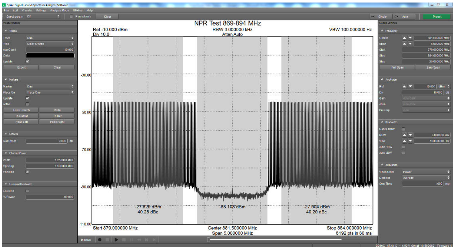
Figure 2: VSG25A 1001-tone, 25 MHz span NPR test noise floor with BB60C. Center 5 MHz shown.
