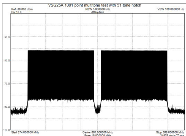
Figure 1: VSG25A test signal for NPR testing
