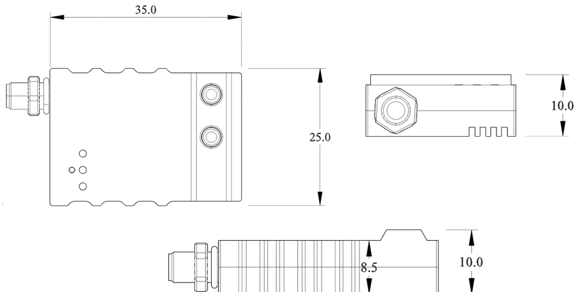
Figure 2: Mechanical drawing
